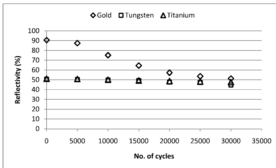
Fig. 6. Reflectivity of abraded metal samples
