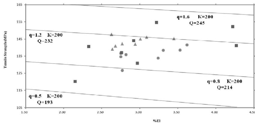
Fig. 5. The quality index chart plotted with the constant value of K equal to 200 MPa for iso-q lines. The squares, circles and triangles represent test bars cast with no, 10 ppi and 20 ppi ceramic foam filter in the runner.
