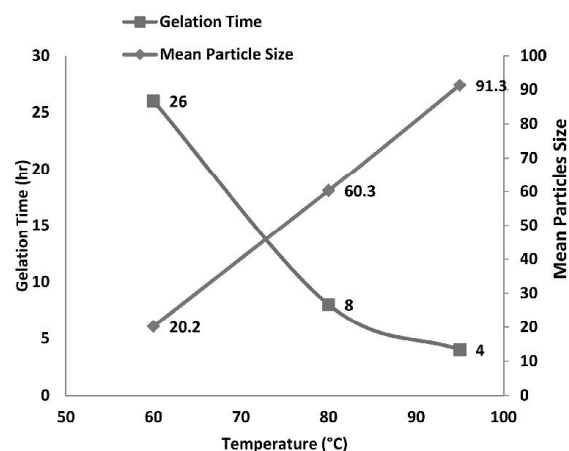
Fig. 5. Effects of temperature on gelation time and mean size of \text{Si}(\text{OH})_4 particles.
