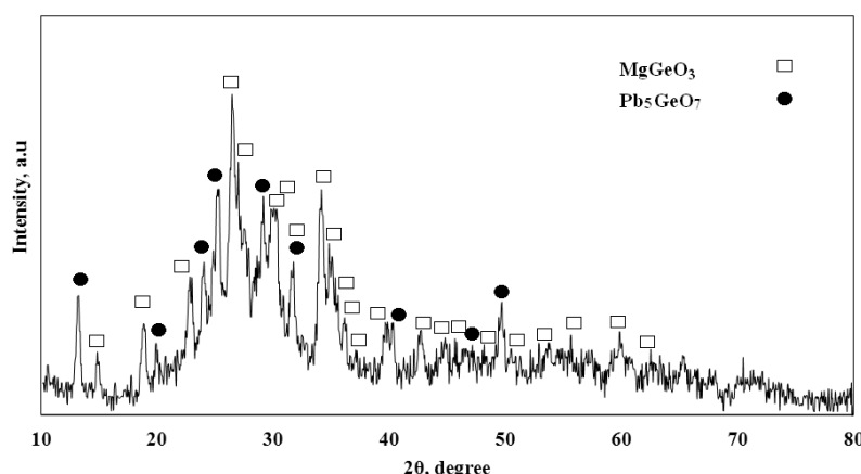
Fig. 4. The XRD pattern of as-quenched 65GeO 2 .15PbO.10MgO.10MgF 2 sample after annealing at 800 °C for 60 minutes.
