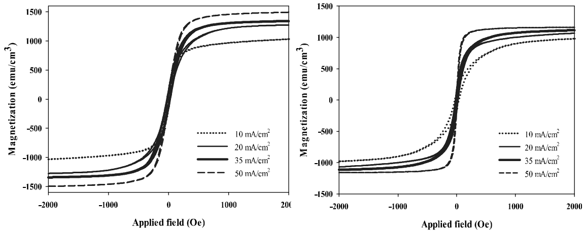
Fig. 6. Hysteresis loops of the coatings obtained from different current densities for (a) pH=5 and (b) pH=3.
