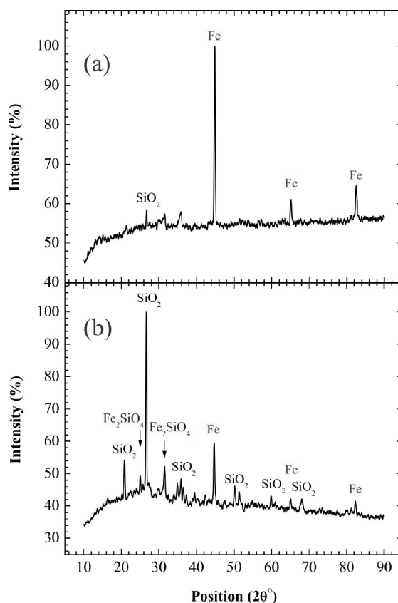
Fig. 7. XRD patterns of the sample with maximum reduction degree (96%), reduced under final optimal conditions (1050°C, 1 hour, 9%lime, 125% of stoichiometry value of required coal for complete hematite reduction). (a) Magnetic part and (b) Non-magnetic part after magnetic separation.
