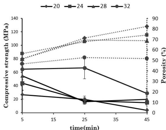
Fig. 10- Strength-porosity variation of specimens with soaking time in the presence of %2wt SiC at 850^\circ\text{C} .
