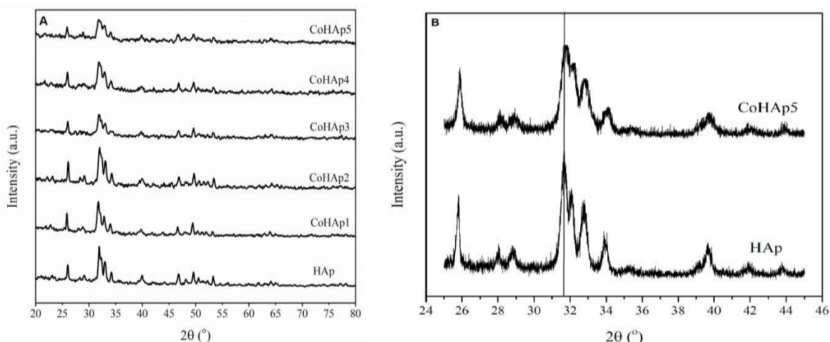
Fig. 1. (A) X-ray diffraction pattern of synthesized HAp, CoHAp1, CoHAp2, CoHAp3, CoHAp4 and CoHAp5 (B) X-ray diffraction pattern of HAp and CoHAp 5 in the 2-theta range of 24-46 with step size of 0.005
